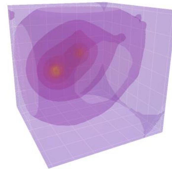
Ground Truth Dark Matter Field
