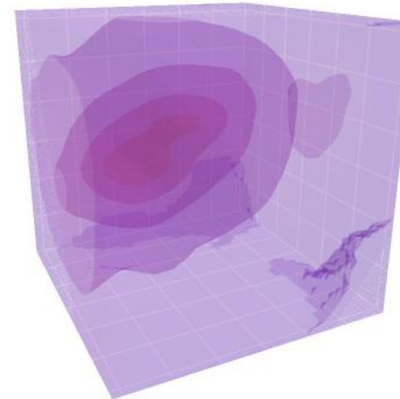
Recovered Dark Matter Field
